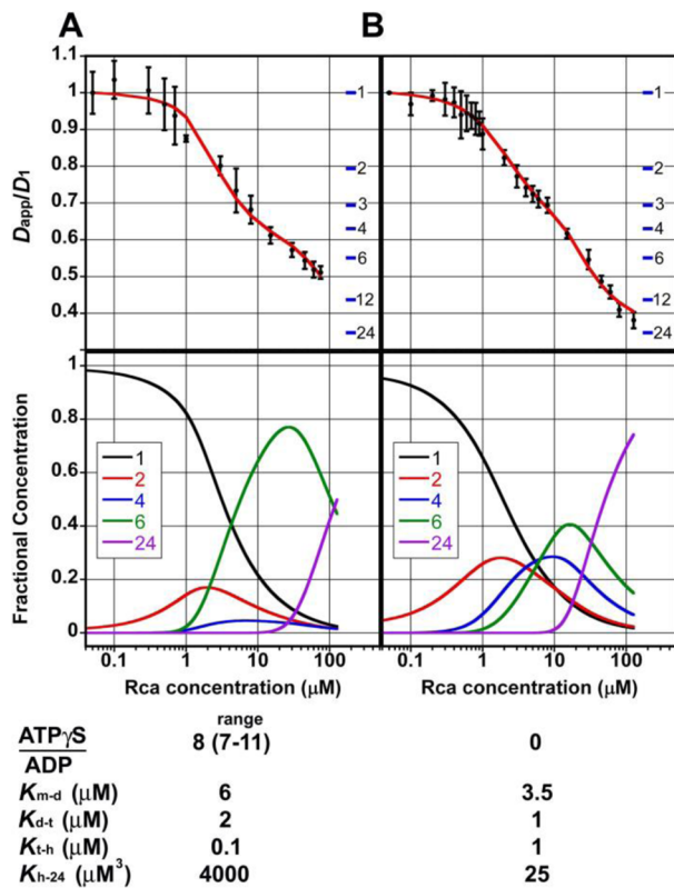
Figure 1. Assembly mechanism of \beta -Rca-AC as a function of ATP \gamma S and ADP. (top) Relative apparent diffusion coefficients ( D_{app}/D_1 ) of \beta -Rca-AC determined by FCS as a function of subunit concentration (black circles). Each sample was prepared in buffer containing 25 mM HEPES–NaOH, pH 7.6, 250 mM KCl, 5 mM MgCl 2 , 10% glycerol, and 2 mM ATP \gamma S (A) or 2 mM ADP (B). For panel A, the ATP \gamma S/ADP ratio was estimated to be 8 (range 7–11) during FCS data collection. The data shown in panel B have been published previously 34 and are replotted for ease of comparison. The horizontal blue lines are placed at calculated values of D_{app}/D_1 for k = 1, 2, 3, 4, 6, 12 , and 24, where k represents the number of subunits per assembly. The red curves represent computer simulations of the Rca assembly mechanism calculated using the K_d values shown in the table below. (bottom) Fractional concentrations of oligomeric species as a function of Rca subunit concentration, as calculated from the K_d values determined by manual curve fitting.
