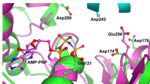
Figure 6. Structural superimpositions of nucleotide-bound FtsH and tobacco Nt-apo- \beta -Rca. (magenta) Cartoon depicting the structure of the AMP-PNP-bound AAA+ module from FtsH (PDB ID 1IY0). The ATP analog AMP-PNP and the catalytic Glu256 of the Walker B motif are represented in ball-and-stick format. (green) AAA+ module of Nt-apo- \beta -Rca (PDB ID 3T15) with the catalytic Asp174 of the Walker B motif and additional conserved acidic residues (Glu121, Asp176, and Asp288) represented in ball-and-stick format. (cyan) Adjacent Nt-apo- \beta -Rca protomer at the crystallographic interface showing the proximity of conserved Asp242 (side chain modeled to C \beta only) to the nucleotide binding pocket. Figure prepared with the PyMOL Molecular Graphics System, Schrödinger, LLC.
